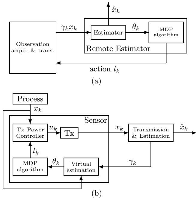
Figure 3: Implementation of the system. The block “Observation acqui. & trans.” in (a) corresponds to the blue-dashed rectangle in Figure 1 and the block “Transmission & estimation” the red-dashed rectangle. In (a), the MDP algorithm is implemented at the remote estimator and the action l_k is fed back to the sensor. While in (b), the MDP algorithm is implemented at the sensor node and \gamma_k is fed back by the remote estimator.
