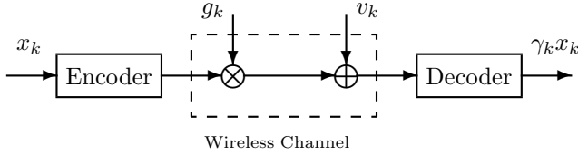
Figure 2: Wireless communication model, where g_k is a random complex number, and v_k is additive white Gaussian noise.
