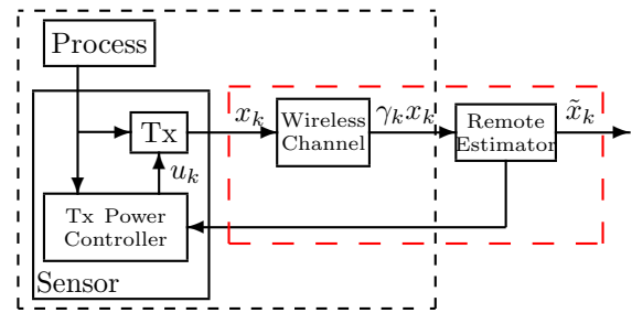
Figure 1: The remote state estimation scheme.
