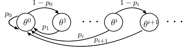
Figure 4: Evolution of belief states under the policy \mathbf{d}(d) with d(\theta, h) \triangleq a_{\theta, h}(e) . The special state \theta^0 = \mathbf{f}_w , p_i = \varphi(\theta^i, h, a_{\theta^i, h}) , \forall i \geq 0 is the successful transmission probability defined just above (16), and \theta^{i+1} = \phi(\theta^i, h, a_{\theta^i, h}, 0) , \forall i \geq 0 , where \phi is the belief state update rule defined in (16). When the belief state is \theta^i , it incurs cost C(\theta^i, h, a_{\theta^i, h}) .
