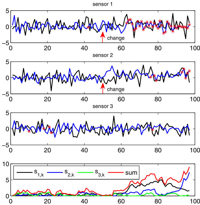
Fig. 4. Typical evolution of the MOS-CuSum algorithm. The top three plots are plotted as in Fig. 3: the black curve represents the observation X_{m,k} , the blue one represents the observation Y_{m,k} and the red stars are used to indicate when the observation Y_{m,k} is sampled.
