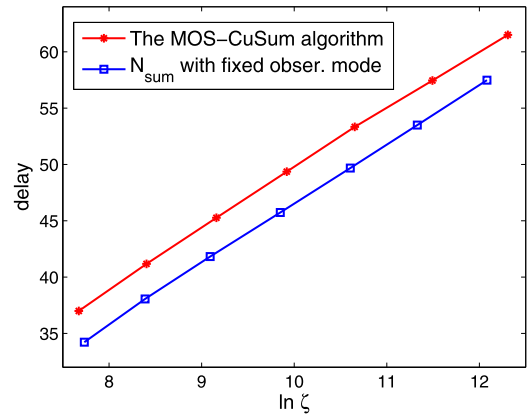
Fig. 6. Detection delay versus the ARLFA for the MOS-CuSum algorithm.
