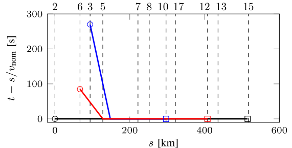
Fig. 8. Platoon plans for a coordination leader (black) and two coordination followers (blue and red) that catch up with the coordination leader to form a platoon. The graph shows the time gap to the platoon leader as a function of the position on the road, where this position is taken along the routes of the individual vehicles. The dashed lines denote the position of the nodes representing road intersections in Fig. 7, with the top labels denoting the node number. As an example, note that the coordination leader starts from Norrtälje (node 2) and drives to Trollhättan (node 15). When the time gap is zero and the routes of the vehicles overlap (between nodes 5 and 10), the vehicles operate in a platoon.
