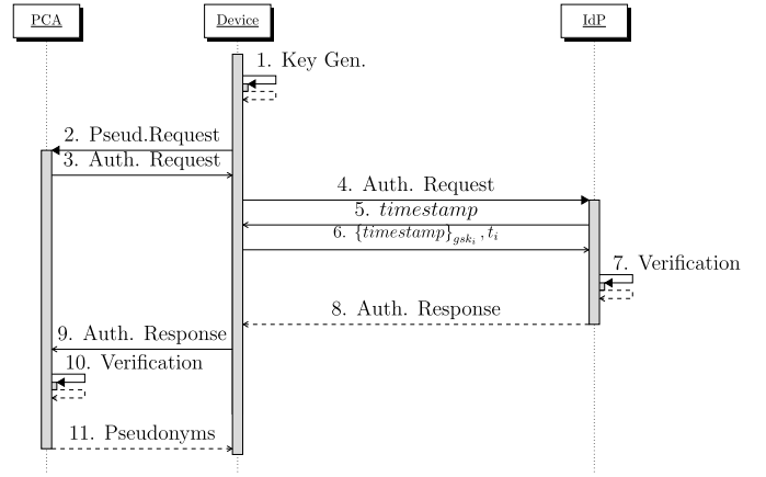
Fig. 2. Authentication protocol.
