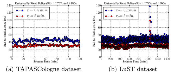
Figure 4: End-to-end latency for P3, \Gamma_{P3}=5 minutes
