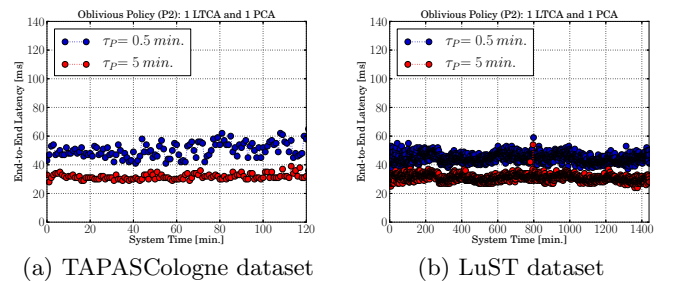
Figure 3: End-to-end latency for P2, \Gamma_{P2}=5 minutes
