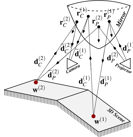
Fig. 1: Representation of the proposed system for the estimation of the depth information: a projector, a RGB camera, and a quadric mirror.
