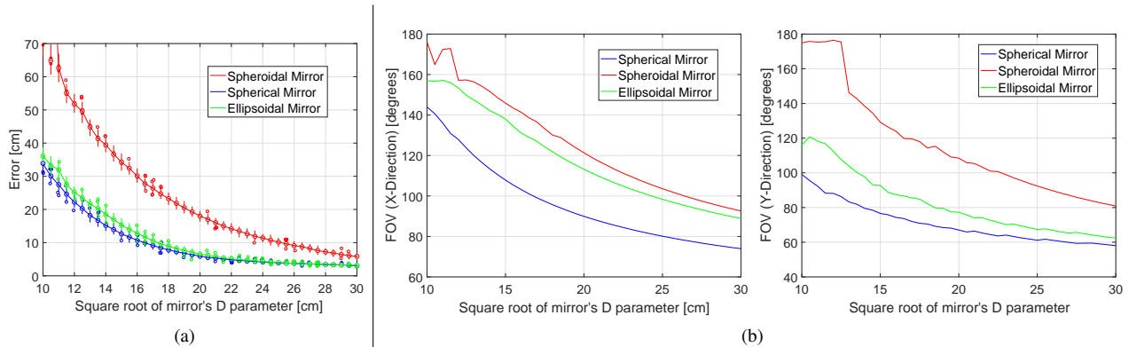
Fig. 7: The influence of the mirror's D parameter (mirror's size – radius in case of the spherical mirror). in the 3D reconstruction (a) and FOV (b).
