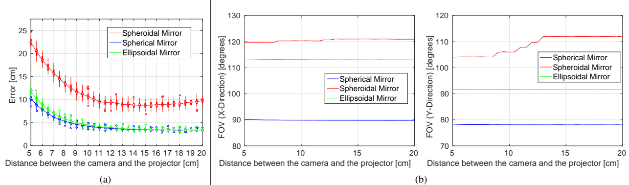
Fig. 8: The influence of the distance between the camera and the projector in the 3D reconstruction (a) and FOV (b).
