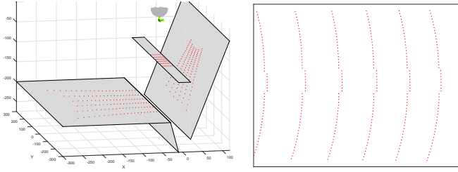
(a) Example of a world and the respective projected pattern. (b) Projection of the pattern onto the camera's image.
