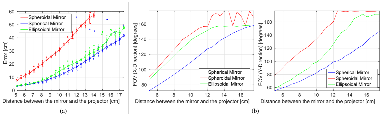
Fig. 9: The influence of the distance between the mirror and the projector in the 3D reconstruction (a) and FOV (b).
