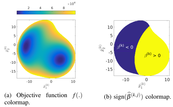
Fig. 3: Example of the variation of the values of the objective function (15), considering the parameters A = 1.59 , B = 1 , C = 35 , D = 25^2 .
