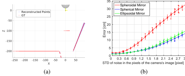
Fig. 6: How the discretization and noise in the position of the pixels in \mathcal{C}(u, v) affects the final results: (a) no discretization or noise in the process (when the reconstruction has no error only the GT points are visible); (b) the influence of discretization and noise in the 3D reconstruction.
