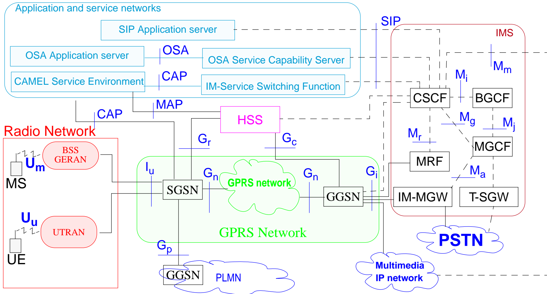
Figure 41: All-IP Architecture
