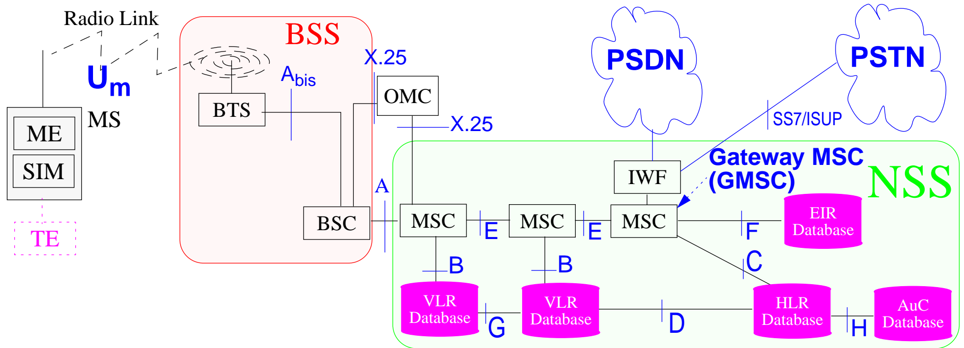
Figure 27: GSM Architecture
