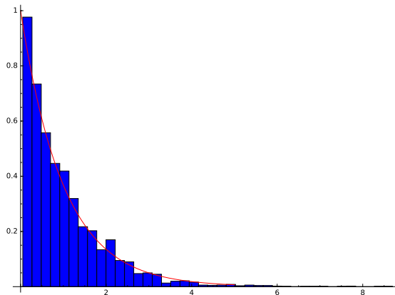
FIGURE 1. Rescaled gaps between consecutive energy levels in [10^{99}, 10^{99} + 110000] , after removing degeneracies. The rescaled gaps have mean one; without rescaling the mean gap is 19.42 \dots . Number of gaps: 5663. We also plot the density function (red in color printout) P(x) = e^{-x} , consistent with Poisson spacings.
