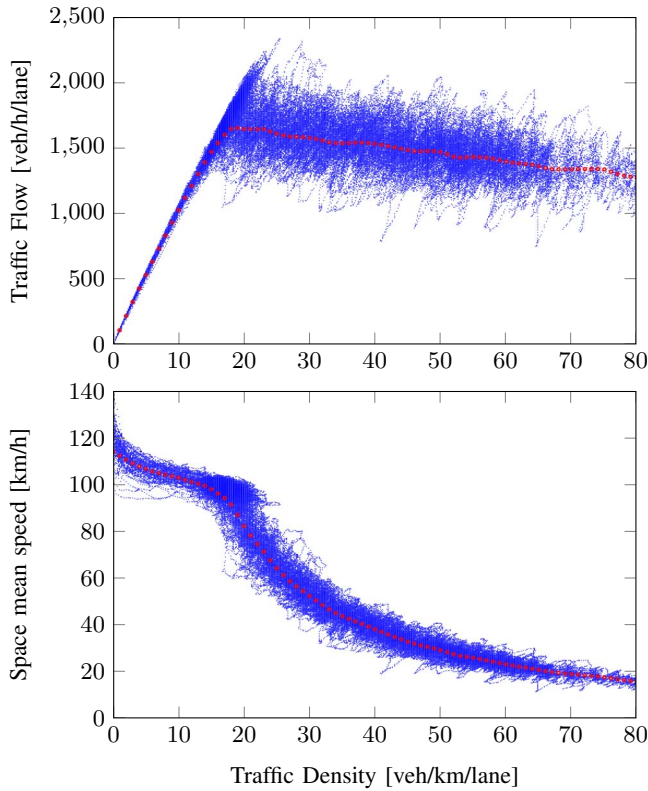
Fig. 6. The fundamental diagram of the two-lane road with a maximum traffic flow of 1650 veh/h/lane, which corresponds to traffic density of 19 veh/km/lane. The blue data points are the simulated results while each red data point is the average of all blue data points between i and i + 1 where i is an integer number of the traffic density.
