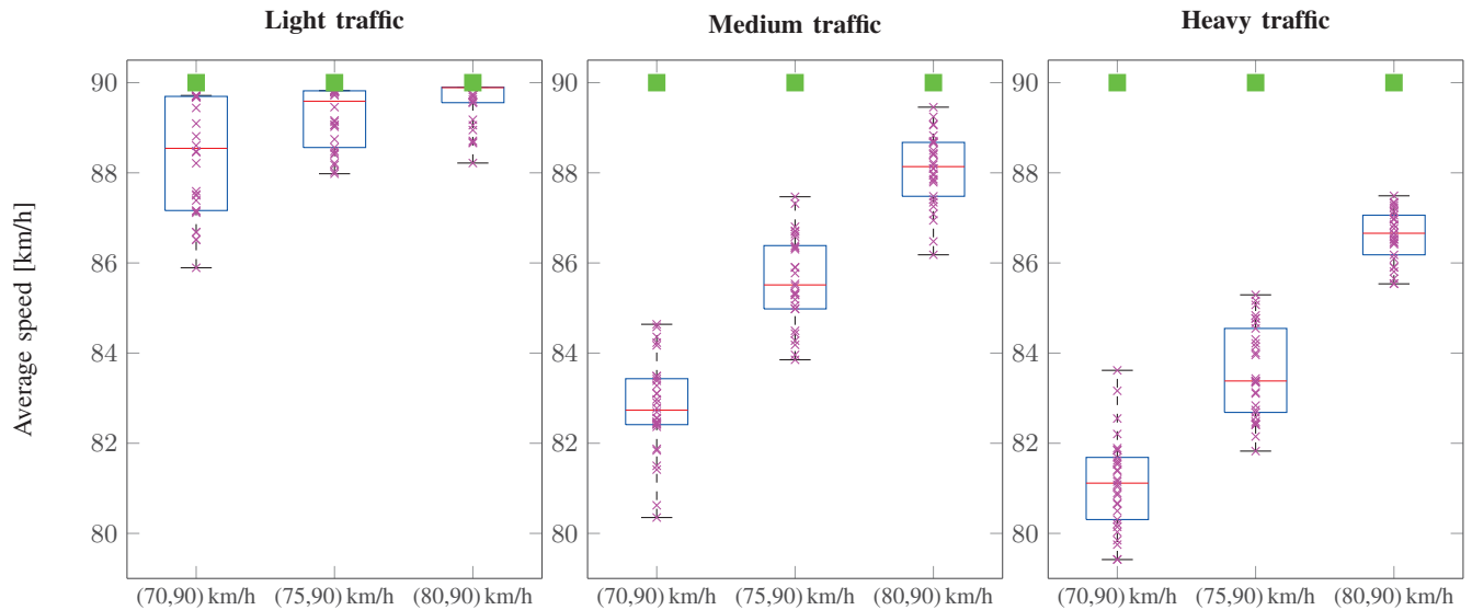
Fig. 9. Box plot of the average speed the trailing HDV had for light (left), medium (middle), and heavy traffic (right). Each individual simulation result are plotted with purple "x". The ideal trailing HDV speed is depicted with a green square. As the traffic density increases, the lower the average speed the trailing HDV could maintain.
