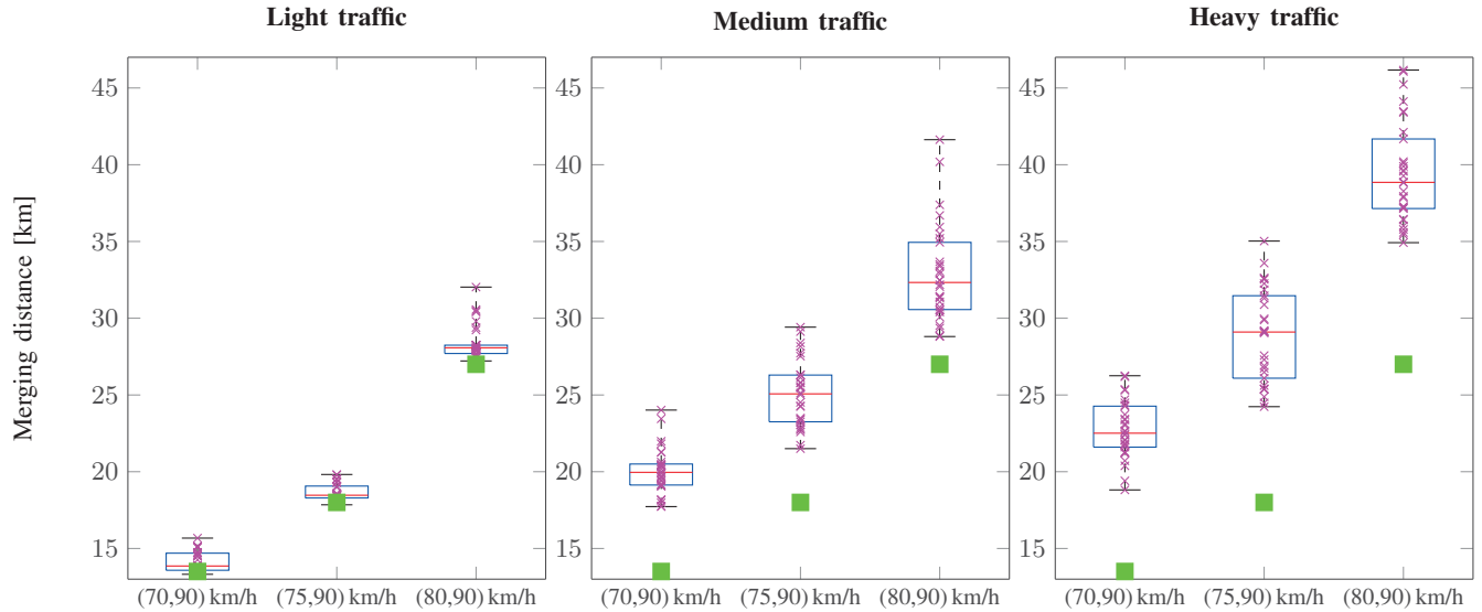
Fig. 8. Box plot of the merging distances for light (left), medium (middle), and heavy traffic (right). Each individual simulation result are plotted with purple "x". The ideal merging distances are depicted with a green square.
