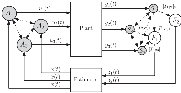
Fig. 1. Networked control system with a network of sensors S_1 , S_2 , and S_3 ; aggregator nodes F_1 and F_2 , and actuators A_1 , A_2 ; and A_3 . Sensors and actuators are responsible for reconfiguring themselves when system failures occur.
