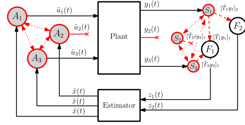
Fig. 4. Networked control system with distributed sensor and actuator reconfiguration. Faults are detected by the sensors and actuators, which are responsible for the reconfiguration. Reconfiguration is achieved through the communication among sensors and among actuators in a distributed manner through the sensor and actuator network, respectively.
