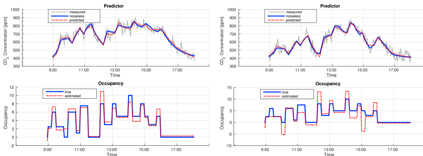
Fig. 5. True (noiseless) and predicted (from the identified model) CO 2 and occupancy signals. Left: database kth_mowc (medium occupancy and closed windows), Tuesday. Right: database kth_mowo (medium occupancy and open windows), Tuesday.
