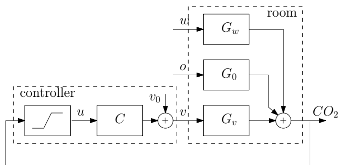
Fig. 4. Block scheme of room dynamics and control architecture. The CO 2 dynamics are driven by the ventilation v , the occupancy o and window opening w . The measured CO 2 is the input to a controller constituted by two blocks in cascade. The first one is a static saturation, the second one is a linear filter denoted by C .
