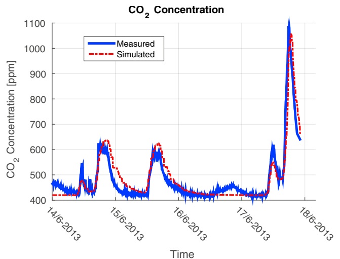
Fig. 2. Validation of the IDA-ICE model. CO 2 levels from room measurements and from simulation are compared.
