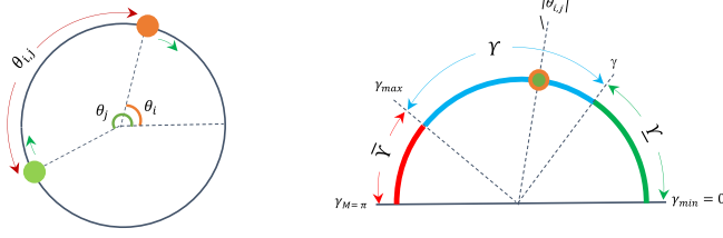
Fig. 1. Relative phase of two oscillators i and j and its map on the arcs \underline{\gamma} , \Upsilon , and \bar{\Upsilon} .
