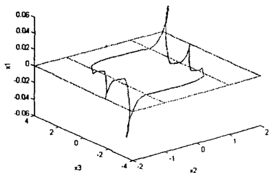
Figure 3: Phase space diagrams of a 3-sliding orbit.
