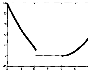
Figure 1: Bifurcation diagram of system (1)–(3), when \rho is varied. The second component of the Poincaré map is plotted against \rho .
