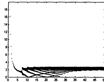
Figure 4: Bifurcation diagram of a sliding orbit showing the second component of the Poincaré map as \rho is kept constant and \omega is varied. Notice the appearance of several fingers corresponding to additional sliding sections.
