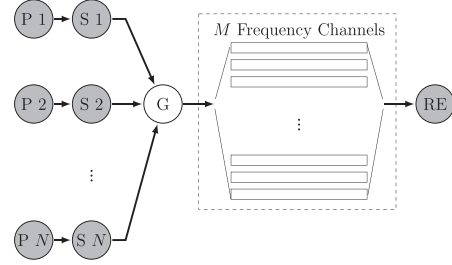
Fig. 1. Multisensor-multichannel remote estimator with a single gateway. Processes, sensors, gateway, and remote estimator are denoted as P_1, P_2, \dots, P_N, S_1, S_2, \dots, S_N, G , and RE , respectively.
