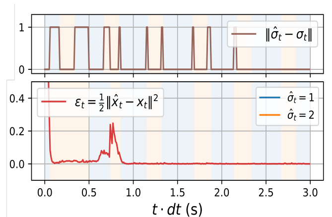
Fig. 5: Identification error over time for system (54). The estimated modes are also compared against the original modes.
