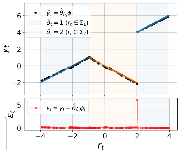
Fig. 3: Identified modes, predicted output and identification error with respect to the true model (52).
