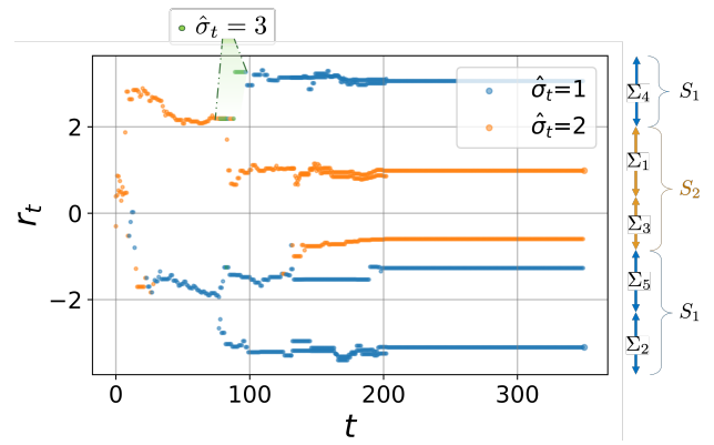
Fig. 2: Evolution of the codevectors \{\hat{\phi}_i\} generated by Alg. 1 for system (52) illustrating the bifurcation phenomenon described in Section IV-B. The association of each effective codevector with each identified mode according to the rule (35) is also shown. Notice that a third mode is detected and quickly discarded as explained in Section IV-C
