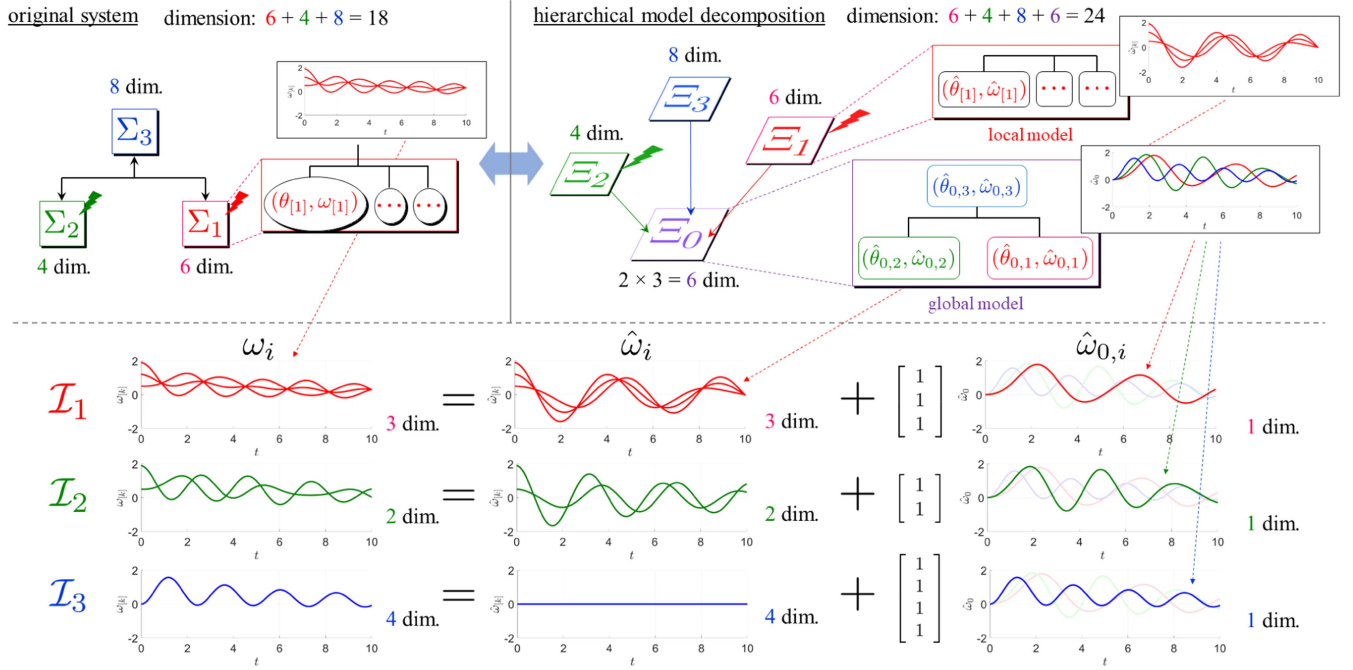
Fig. 4. Hierarchical model decomposition of the second-order network system of the motivating example. (Top) Block diagrams of the original network system and the hierarchical system. (Bottom) Responses of \omega_i in \Sigma_i and their representations as a superposition of \hat{\omega}_i in \Xi_i and \hat{\omega}_{0,i} in \Xi_0 for i = 1, 2, 3 .
