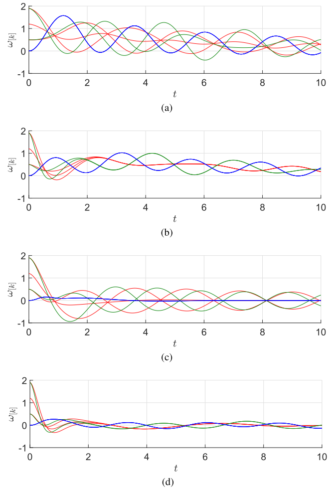
Fig. 8. Responses of the second-order network system with different control policies. (a) Free response. (b) Response only with the local subcontrollers. (c) Response only with the global subcontroller. (d) Response with the global controller.
