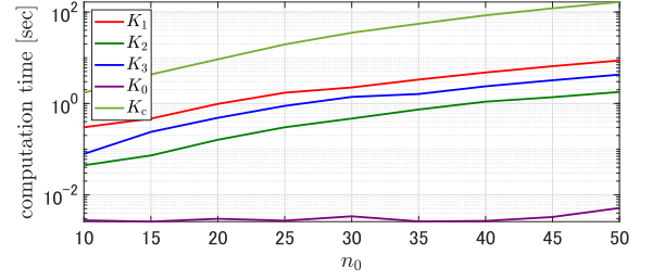
Fig. 9. Average computation times for designing the local subcontrollers K_1 , K_2 , and K_3 , the global subcontroller K_0 , and the centralized controller K_c for varied n_0 ranging from 10 to 50 on a logarithmic scale.
