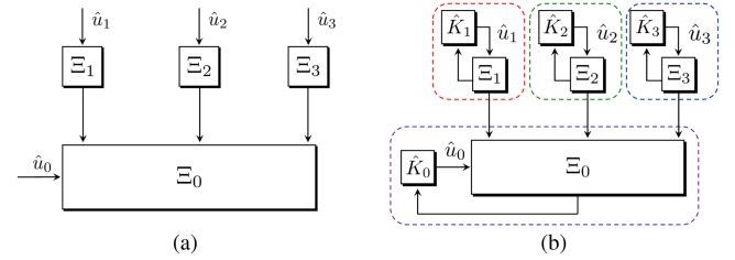
Fig. 5. Block diagrams of the hierarchical model decomposition with control signals. (a) With control inputs. (b) With feedback control.
