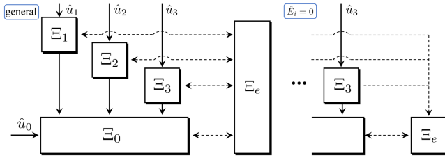
Fig. 7. Block diagrams of the hierarchical model decomposition with error dynamics in (18) when N = 3 . (Left) General case. (Right) Case under choice (20), where the system has a hierarchical structure including the error dynamics.
