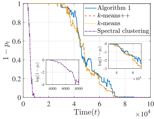
Fig. 3. Performance comparison of four methods.
