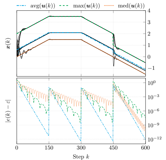
Fig. 1: Evolution of a network, with n = 5 agents in a line configuration, running the protocol in eq. (5) designed with \alpha = 0.5 and \rho = 2 . The parameter \varepsilon denotes the empirical bound on the tracking error e(k) characterized in Theorem 1.
