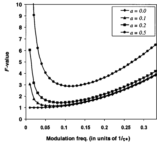
Fig. 3. F -value as a function of modulation frequency for square-wave excitation with different duty cycles a ( a = 0.0 represents Dirac pulses).
