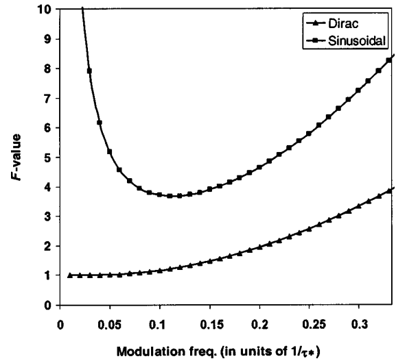
Fig. 2. Normalized relative rms noise F as a function of modulation frequency with lock-in detection. Low F -values represent good performance. Theoretically, F \geq 1 . Curves shown are for excitation by a train of Dirac pulses and sinusoidal excitation.
