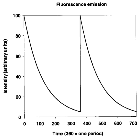
Fig. 1. Fluorescence light intensity as a function of time with excitation by a train of Dirac pulses.
