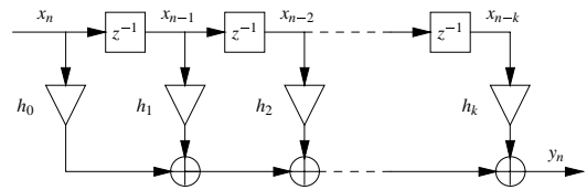
Figure 10: FIR-Filter
