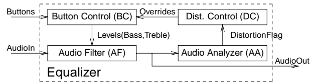
Figure 7: The Digital Equalizer
