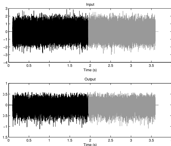
Fig. 4: Measured input and output signal. Black part: estimation data (user available data to build the model); gray part: test data: to be used only for bench marking).
