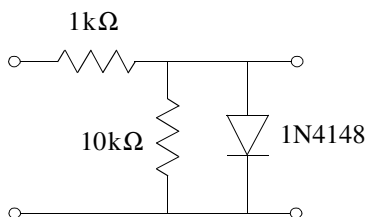
Fig. 2: Circuit used to build the static nonlinear system.
