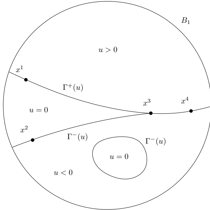
FIGURE 1. x^1 a positive one-phase point, x^2 a negative one-phase point, x^3 a branching point and x^4 a non-branching two-phase point.
