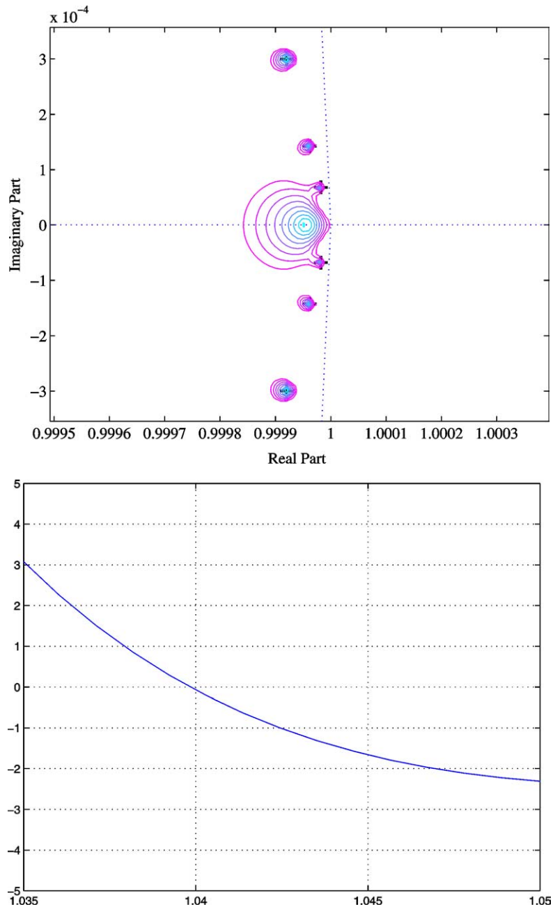
Fig. 2. Level curves of the kernel function K_A^\alpha(\cdot, 0) for the zero set A generated by the parameter values: \alpha = 3 , n = 6 , \theta = 0.51 , d = 10 (top). Values of the kernel function K_A^\alpha(1, 0) for the zero set A generated by the parameters: n = 1500 , \theta = 0.033 , d = 1.045 and 1.035 \leq \alpha \leq 1.050 (bottom).
