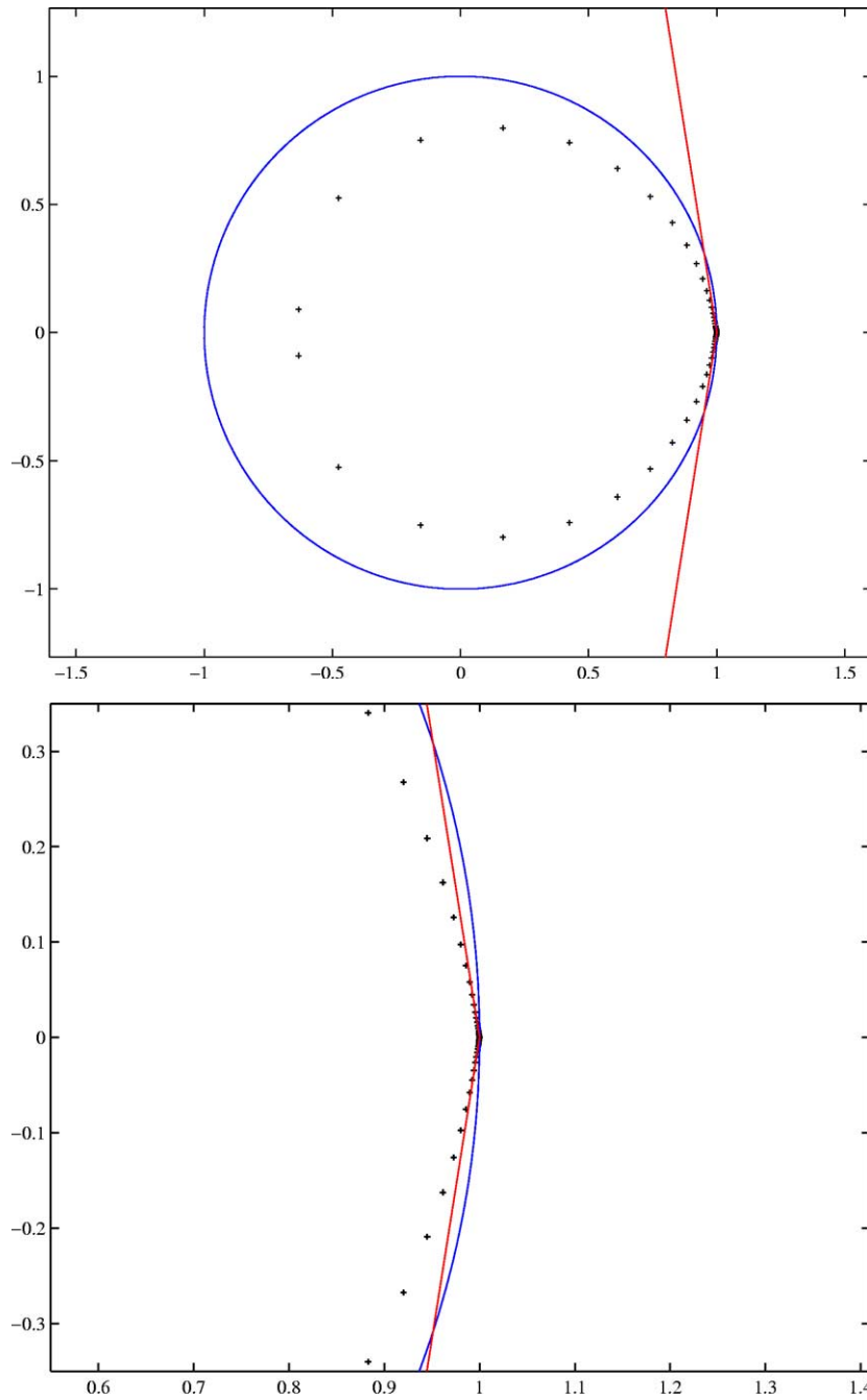
Fig. 1. Zero set A for n = 80 generated by the parameters \theta = 0.15 , d = 1.3 , for \alpha = 1.5 . The indicated straight lines are tangents to the curves on which the zeros are located.
