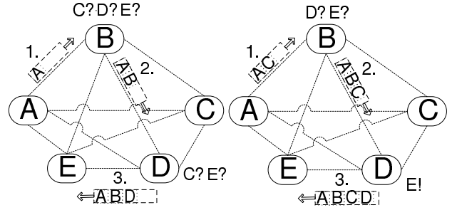
Fig. 1. A simple example of Minstrels with five nodes.
