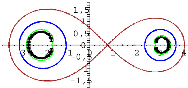
FIGURE 9. Zeros of Bergman polynomials P_n of Example 6.2, for n = 140, 150 and 160 .
