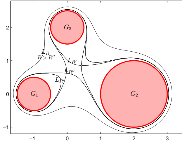
FIGURE 1. Green level curves
