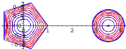
FIGURE 2. Level curves of \Lambda_{100}(x + iy) , on \{(x, y) : -2 \leq x \leq 5, -2 \leq y \leq 2\} , with G as in Example 6.1.
