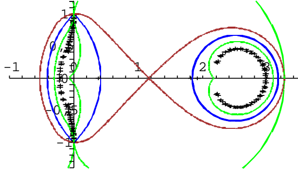
FIGURE 12. Zeros of Bergman polynomials P_n of Example 6.5, for n = 80, 90 and 100 .
