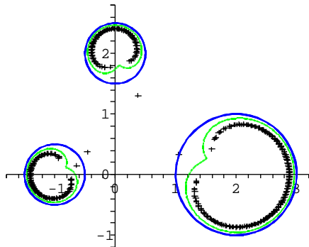
FIGURE 13. Zeros of Bergman polynomials P_n of Example 6.6, for n = 80, 90 and 100 .
