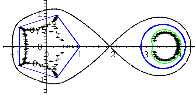
FIGURE 8. Zeros of Bergman polynomials P_n of Example 6.1, for n = 80, 90 and 100 .
