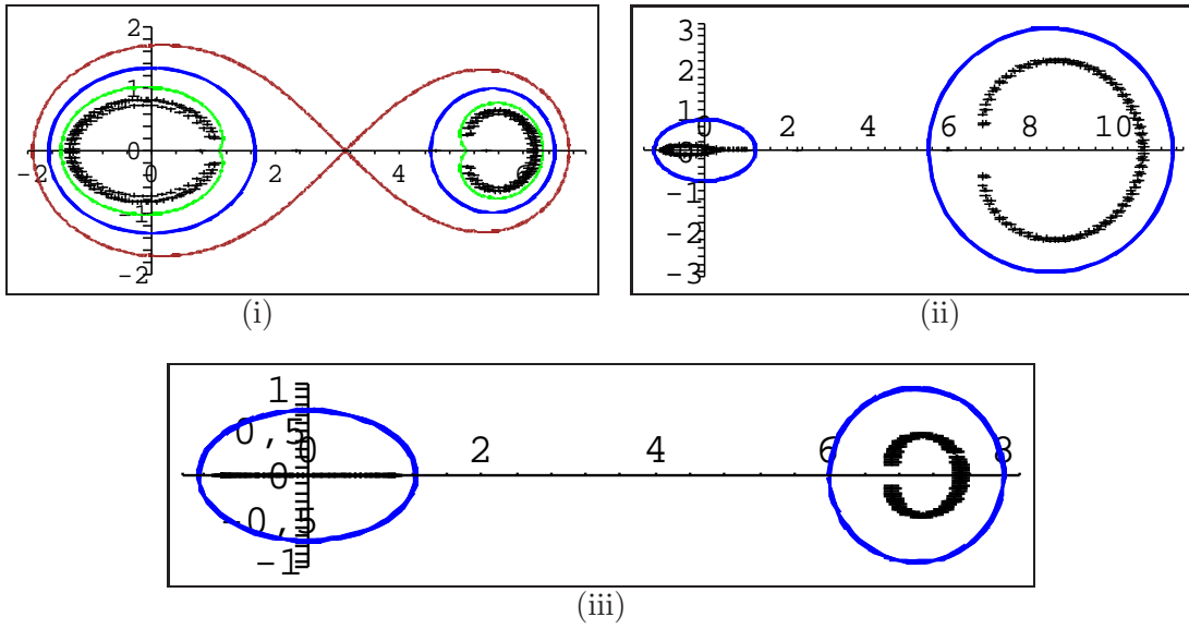
FIGURE 10. Zeros of Bergman polynomials P_n of Example 6.3, for n = 80, 90 and 100 .
