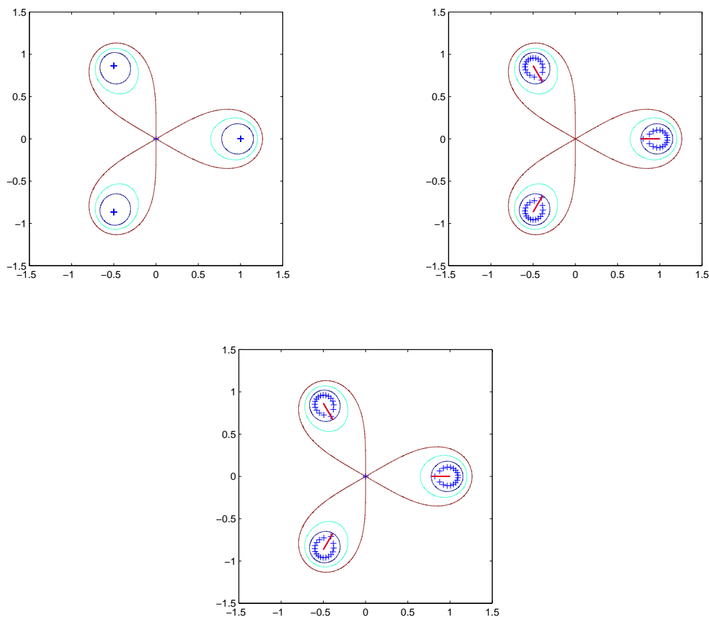
FIGURE 14. Zeros of the Bergman polynomials P_n for the lemniscate case m = 3 and r = 0.9 , for n = 50, 51 and 52 .
