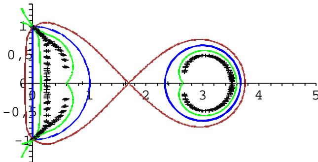
FIGURE 11. Zeros of Bergman polynomials P_n of Example 6.4, for n = 80, 90 and 100 .
