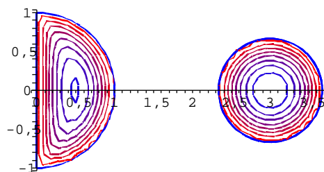
FIGURE 6. Level lines of \Lambda_{100}(x + iy) , on \{(x, y) : -1 \leq x \leq 6, -2 \leq y \leq 2\} , with G as in Example 6.4.
