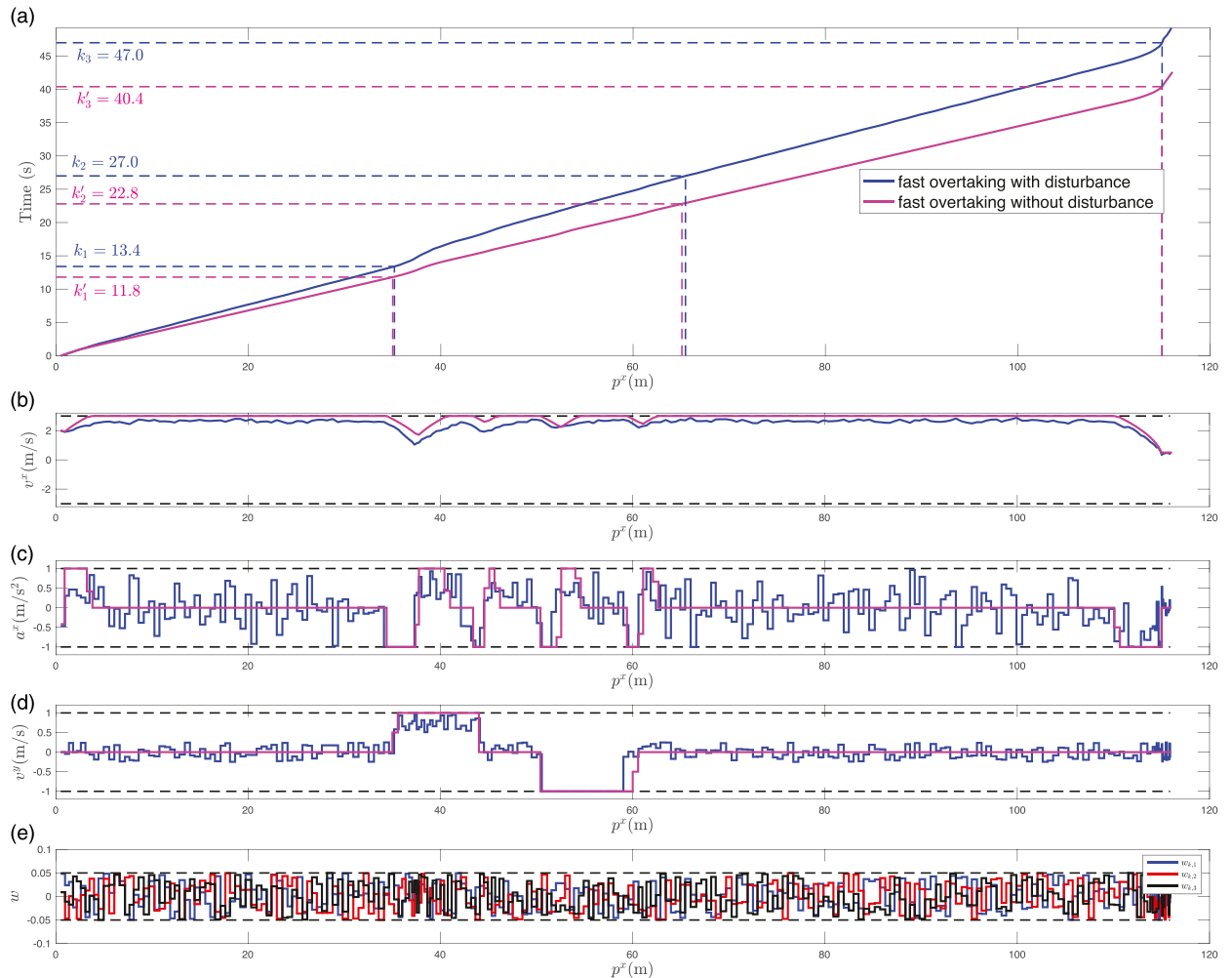
Figure 14. Comparison of robust control with noise and deterministic control without disturbance signal in the fast overtaking: (a) position-time trajectory; (b) velocity trajectory of x-axis; (c) control trajectory of x-axis; (d) control trajectory of y-axis; (e) disturbance signals.
