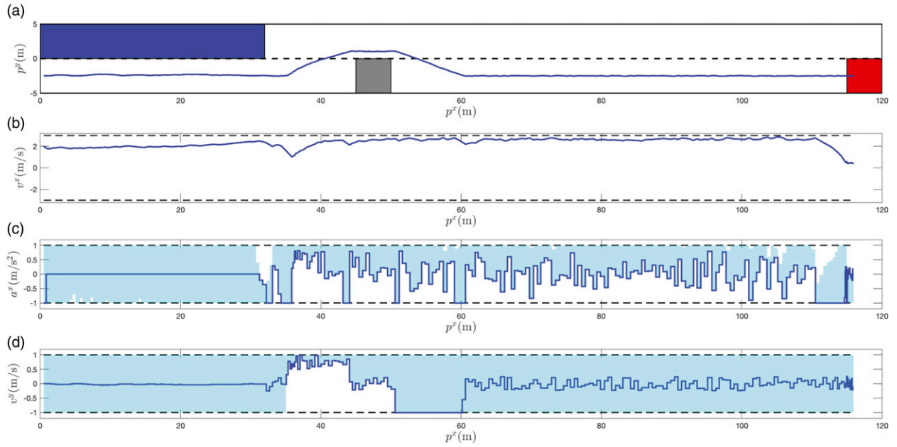
Figure 13. Trajectories for one realization of disturbance signal in the slow overtaking: (a) position trajectory; (b) velocity trajectory of x-axis; (c) control trajectory of x-axis; (d) control trajectory of y-axis.
