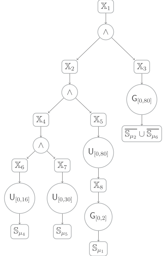
Figure 11. The constructed tTLT \mathcal{T}_{\varphi_{fast\_overtake}} .
