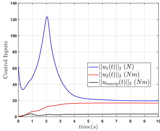
Fig. 8: The evolution of the control input signals \|u_1(t)\|_2 , \|u_2(t)\|_2 and \|u_{manip}(t)\|_2 .
