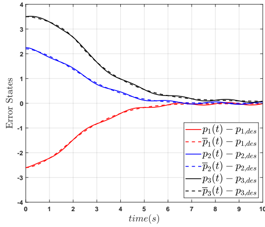
Fig. 7: The evolution of the real position errors of the end-effector p_1(t) - p_{1,d} , p_2(t) - p_{2,d} , p_3(t) - p_{3,d} depicted with solid lines as well as the corresponding nominal position errors \bar{p}_1(t) - p_{1,d} , \bar{p}_2(t) - p_{2,d} , \bar{p}_3(t) - p_{3,d} depicted with dashed lines, for the transition of the UVMS between RoI \mathcal{R}_1 - \mathcal{R}_3 .
