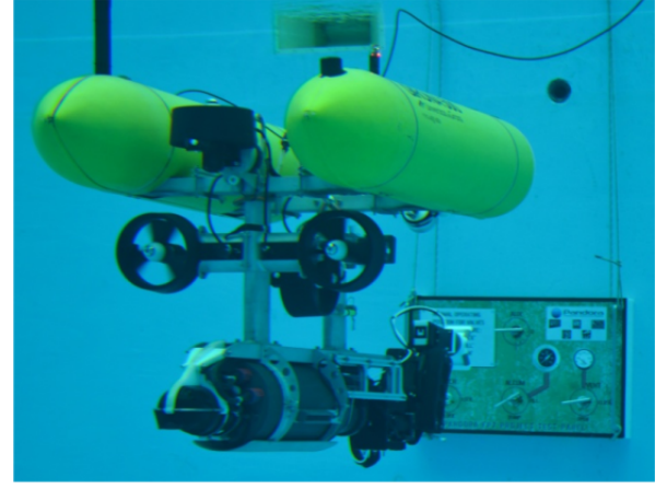
Fig. 4: The GIRONA-UVMS composed of Girona500 AUV and ARM 5E Micro manipulator [7].
