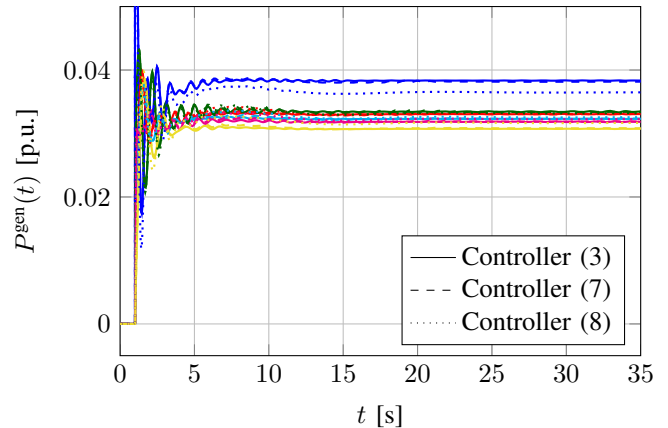
Figure 5: Total generated power in the AC areas for the controllers (3), (7) and (8), respectively.
