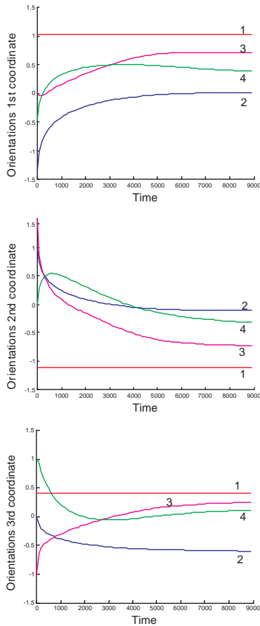
Fig. 1. Time histories of the orientations for the four rigid bodies using the leader-follower structure.
