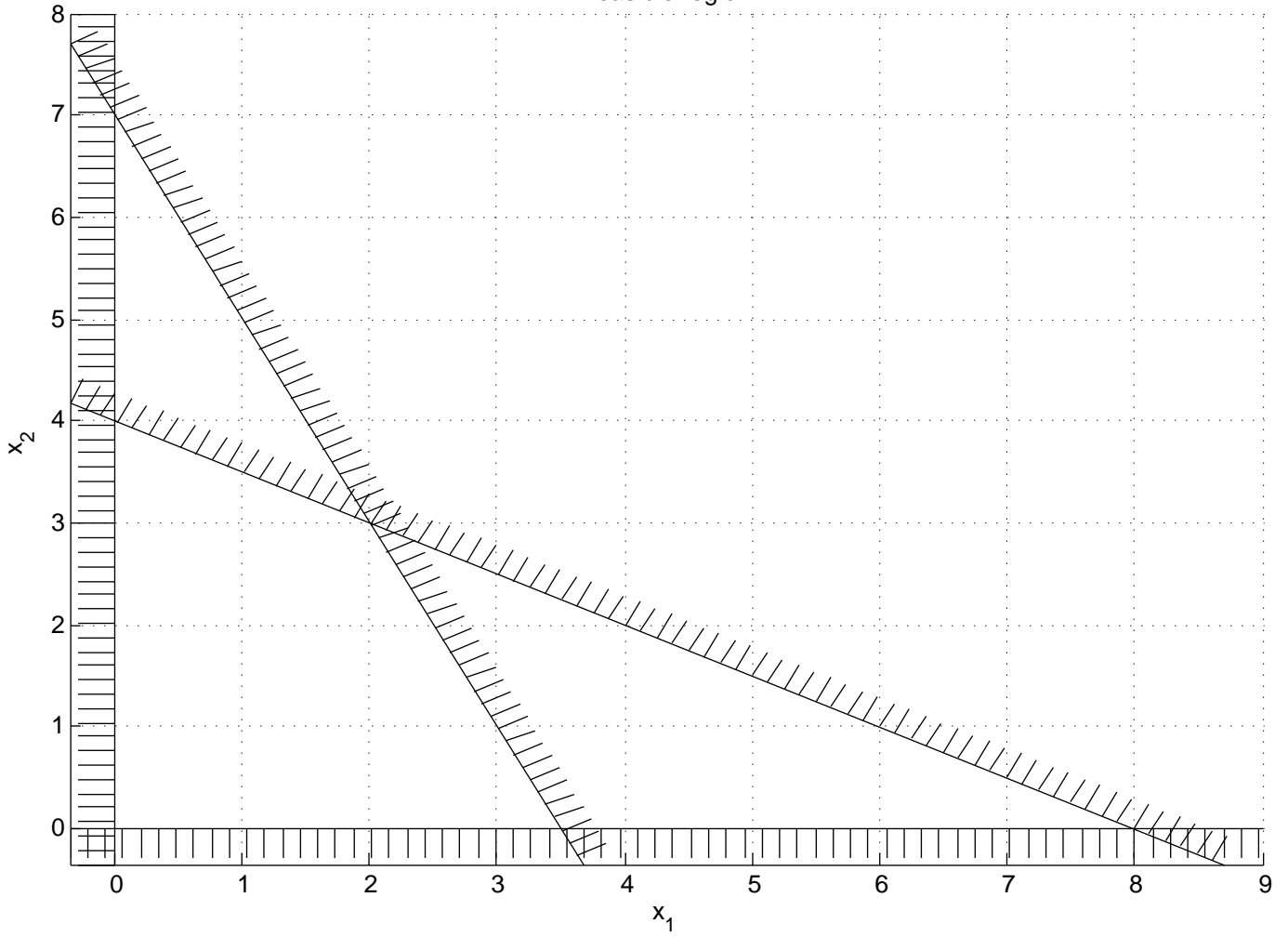
Feasible region
