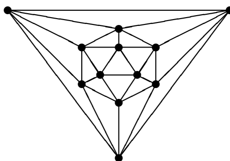
"Ikosaeder" m = 3, n = 5
