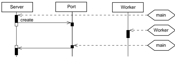
Figure 1. A thread switch from main to Worker, and back.
