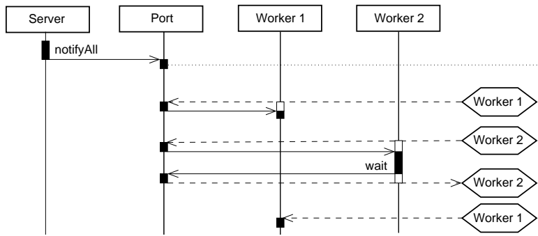
Figure 6. Thread notification: Main thread notifies both worker threads.
