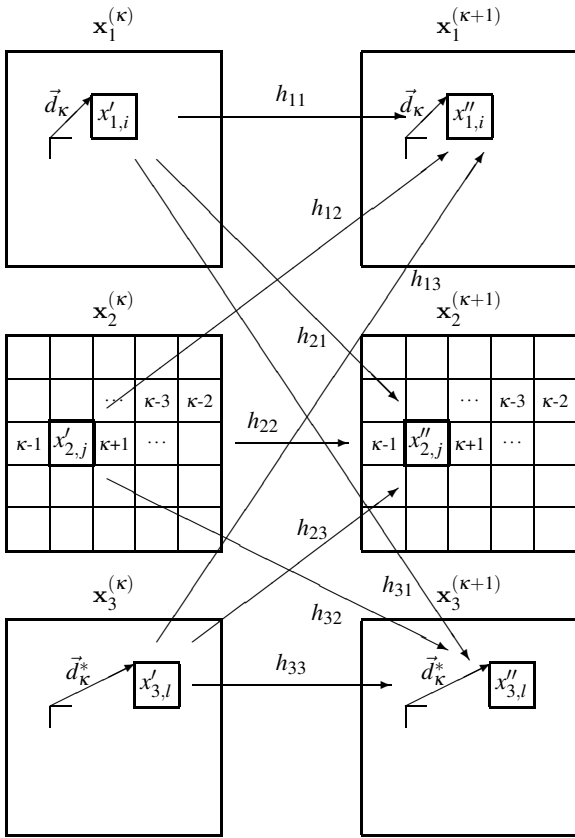
Figure 1: The incremental transform T_\kappa for the three frames \mathbf{x}_1^{(\kappa)} , \mathbf{x}_2^{(\kappa)} , and \mathbf{x}_3^{(\kappa)} which strictly maintains orthogonality for any bidirectional motion field (\vec{d}_\kappa, \vec{d}_\kappa^*) . T_\kappa minimizes the energy in x_{2,j} .
