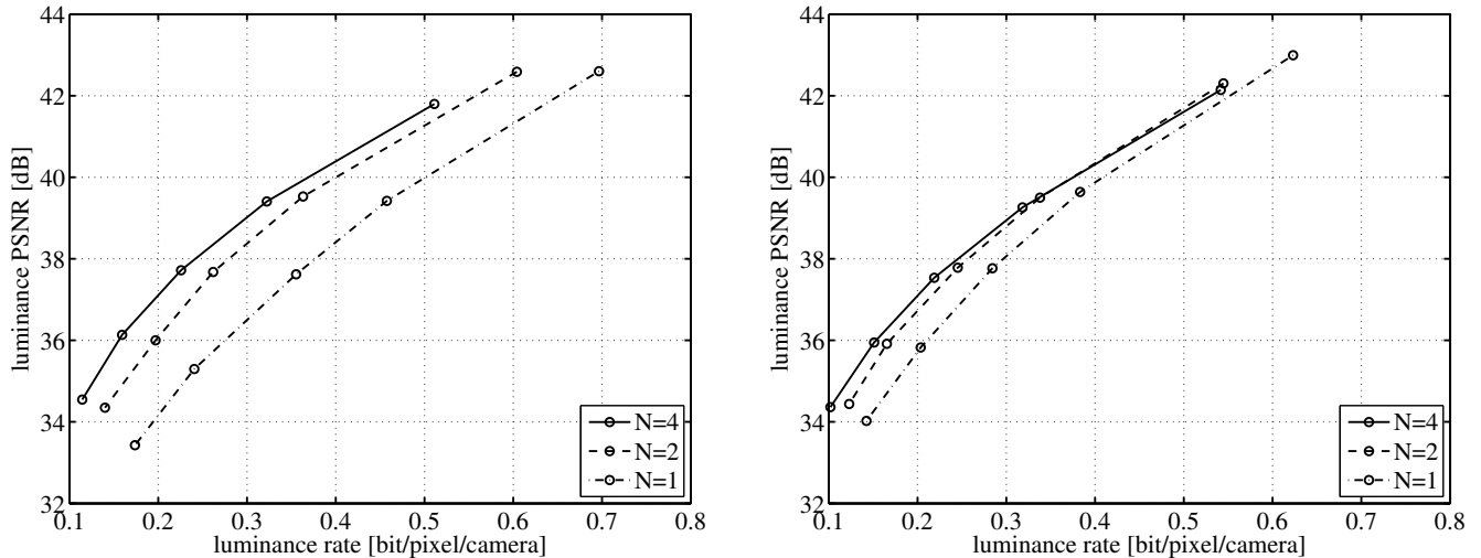
Figure 5: PSNR over bit-rate for the luminance signal of the data set Breakdancers . The performance of view GOP sizes of N = 1, 2, 4 are compared for a temporal GOP size of K = 1 (left) and K = 2 (right).
