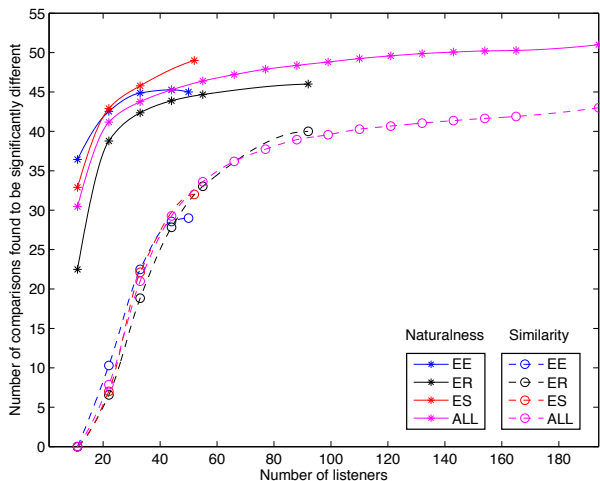
Figure 1: Number of significantly different pairs in MOS tests, as a function of the task and the number of listeners. The theoretical maximum is 55.
