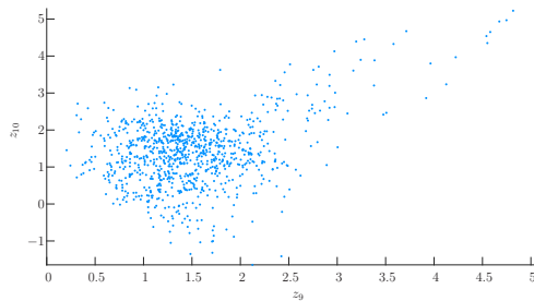
Figure 2: Learned control vectors in Sad emotional subspace. All other point clouds are close to Gaussian in appearance.
