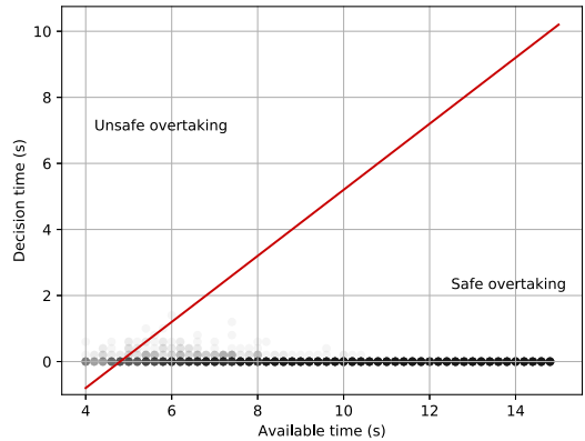
Fig. 4. Scatter plot for the risk-agnostic decision rule with estimator having no prior. The red line marks the border between safe overtakings ( T_o < T_m(t) ) and unsafe overtakings ( T_o > T_m(t) ).
