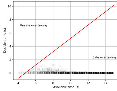
(b) \delta = 0.1, \beta = 0
