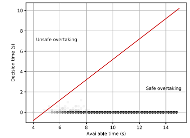
(c) prior \mu_0 = [2\Delta x(0), \Delta v(t)]^T and \Sigma_0
