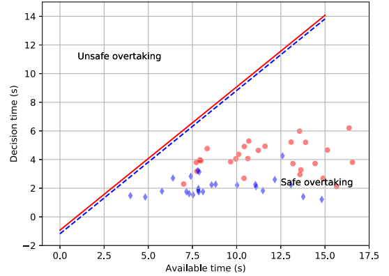
Fig. 11. The “available time-decision time”-diagram for Driver A (red circles) and Driver B (blue diamonds). The line for each subject is determined by the corresponding estimated overtaking time T_o .
