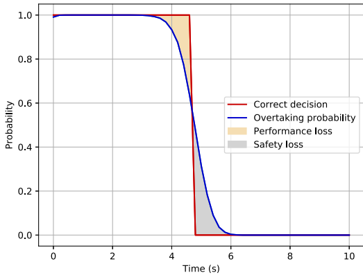
Fig. 3. Probability \mathbb{P}(T_o < \hat{T}_m(t)) that the risk-agnostic decision rule with estimator having no prior grants an overtaking as a function of time in blue, and correct decision \mathbb{1}\{T_o < T_m(t)\} in red.
