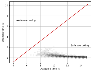
(a) prior \mu_0 = [0, \Delta v(t)]^T and \Sigma_0
