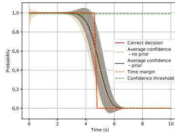
(b) prior \mu_0 = [2\Delta x(0), \Delta v(t)]^T and \Sigma_0
