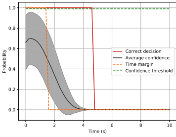
(a) \delta = 0.01 and \beta = 3
