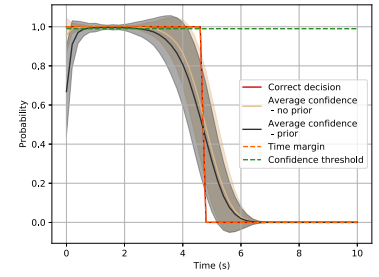
(c) prior \mu_0 = [0, \Delta v(t)]^T and \Sigma_0
