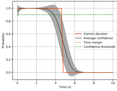
(a) 1000 realizations, \delta = 0.1 and \beta = 0
