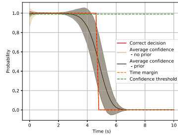
(b) prior \mu = s(0) and \Sigma_0
