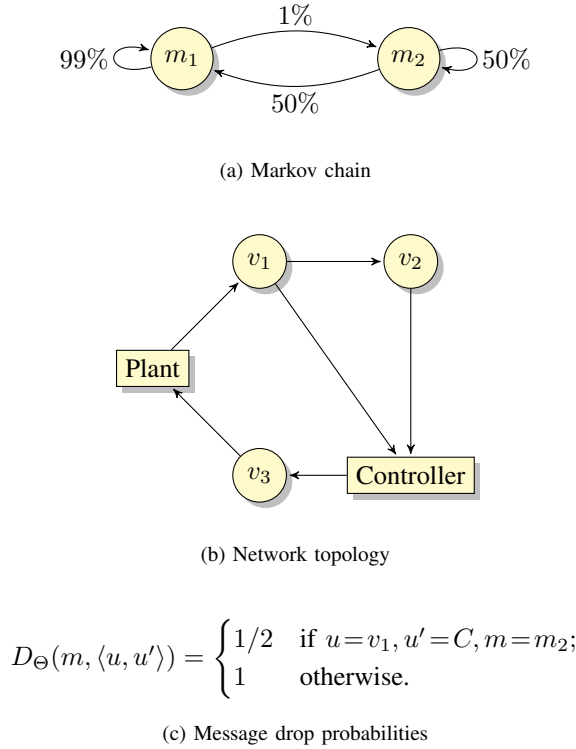
Fig. 3. Example of a system with a Markov link-failures model.
