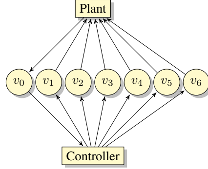
(a) Network topology
