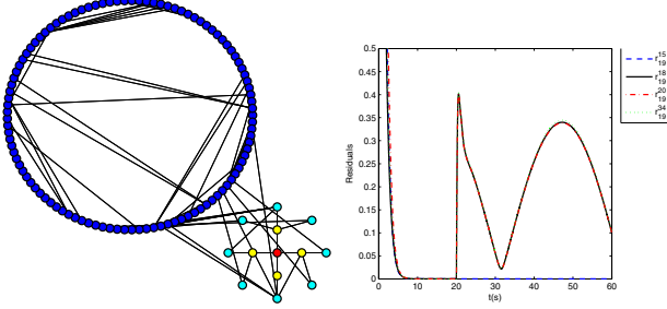
Fig. 3. [left] The graph of the IEEE 118 bus network. Node 19 (red) is the node at the center of the smaller cluster to the right, monitoring its 1-hop neighbours (yellow). This cluster represents the 2-hop neighbourhood of node 19. [right] Residuals generated by the UIO bank at node 19.
